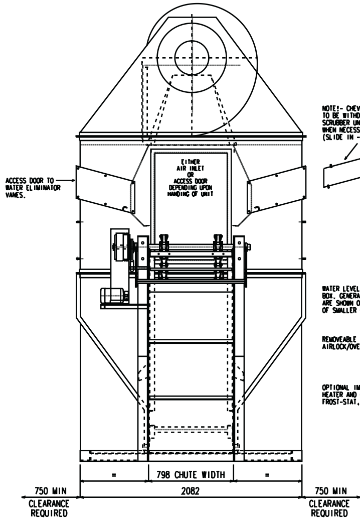
FRONT ELEVATION OF WET COLLECTOR
