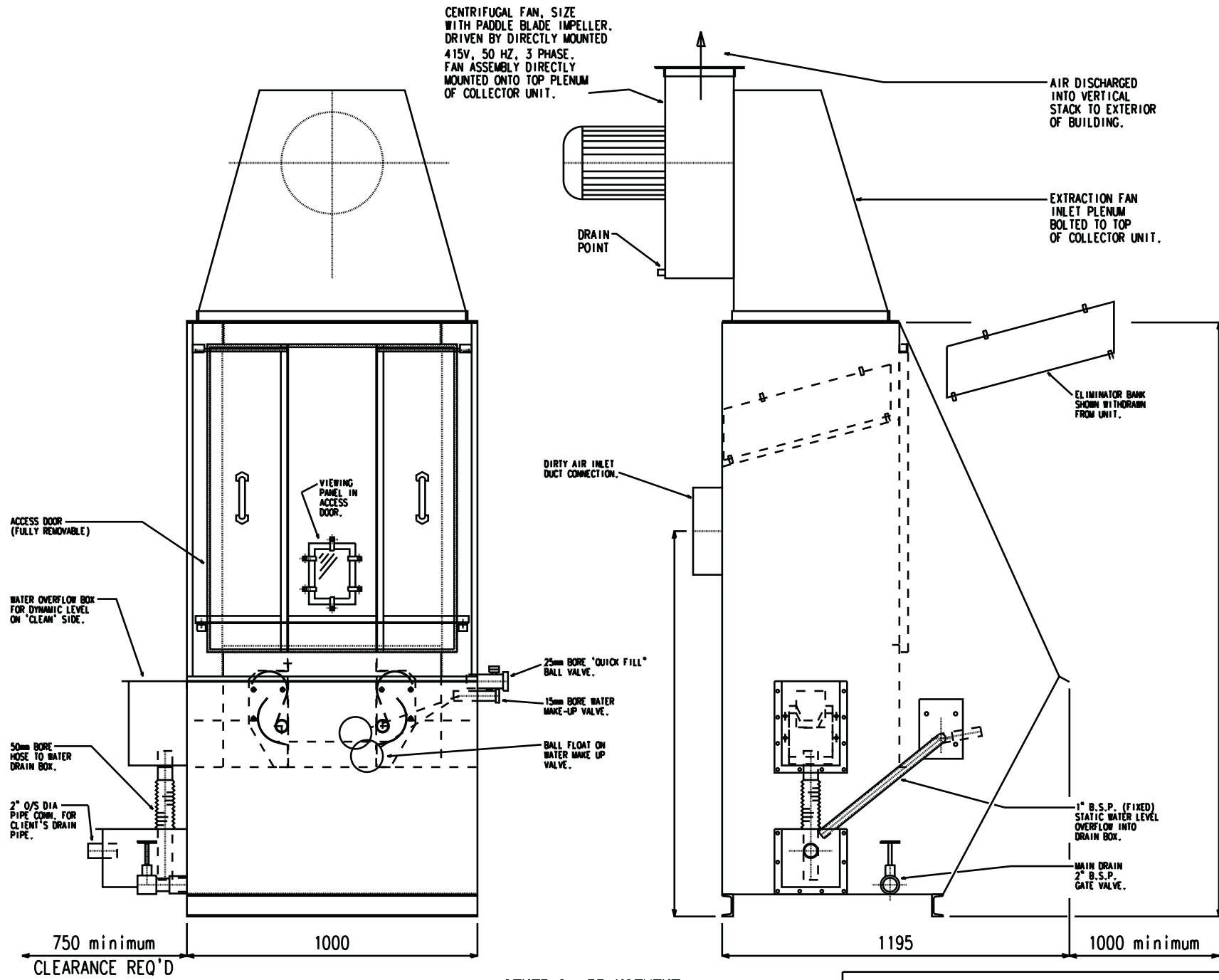
GENERAL ARRANGEMENT OF 2000 CFM DUTY ECONOMY RANGE WET COLLECTOR UNIT
